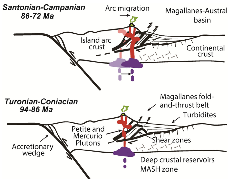
FIG. 7. Schematic reconstruction model for the origin and crustal emplacement of the Petite and Mercurio plutons during the Late Cretaceous stages of Rocas Verdes marginal-basin closure. MASH : Melting, Assimilation, Storage, and Homogenisation.
