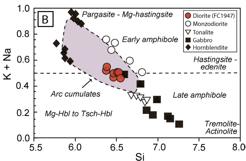
FIG. 6. Si (a.p.f.u) vs Na+K (a.p.f.u) in Ca amphibole diagram. Modified from Torres García et al. (2020), including their compositional database of amphiboles other than for FC1947.
