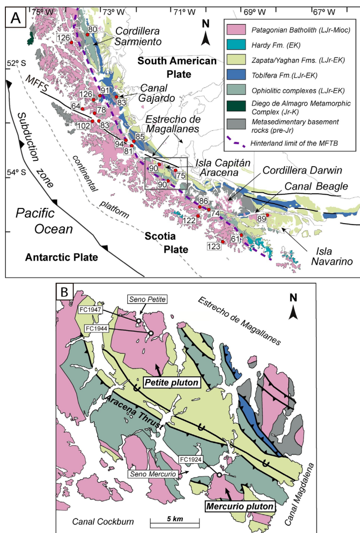
FIG. 1. A. Simplified geological map of the southernmost Andes (modified from Sernageomin, 2003). Zircon U-Pb crystallisation ages are shown (red dots, mean values; data from Hervé et al. , 2007a; Calderón et al. , 2007; Klepeis et al. , 2010; Torres García et al. , 2020; Muller et al. , 2021; Velásquez et al. , 2023). B. Geological map of Isla Capitán Aracena with the locations of samples that were collected from the Petite and Mercurio plutons (see location in A). MFFS : Magallanes-Fagnano Fault System. MFTB : Magallanes Fault-and-Thrust Belt. Jr : Jurassic. K : Cretaceous. LJr : Late Jurassic. EK : Early Cretaceous. Mioc : Miocene.
