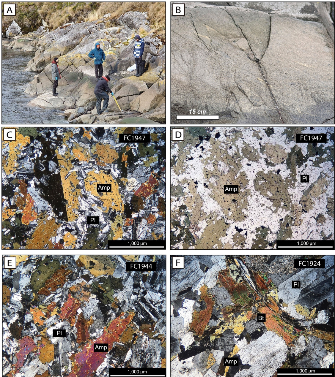
FIG. 2. A. Field photo of the group working on the Petite pluton. B. Medium-grained hornblende diorite of the Petite pluton showing compositional banding with preferred orientation of leucocratic segregations bands. C–F. Photomicrographs of representative areas of samples illustrating the variety of mineral assemblages and textures of analysed samples. Amp: amphibole, Bt: biotite, Pl: plagioclase.
