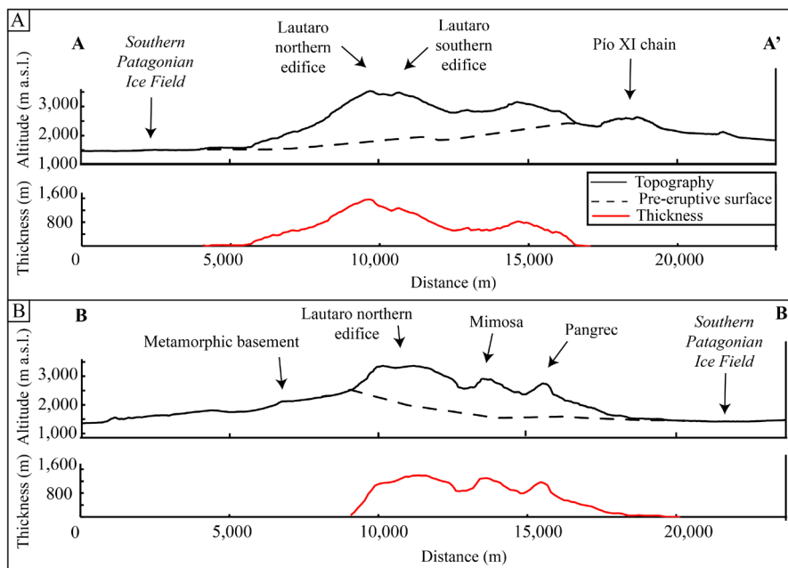
FIG. 3. Topographic, pre-eruptive, and thickness profiles along two transects crossing Lautaro volcano. A. AA' transect (NW-SE oriented). B. BB' transect (SW-NE oriented). See figure 2 for transect locations. See text for pre-eruptive surface acquisition.
