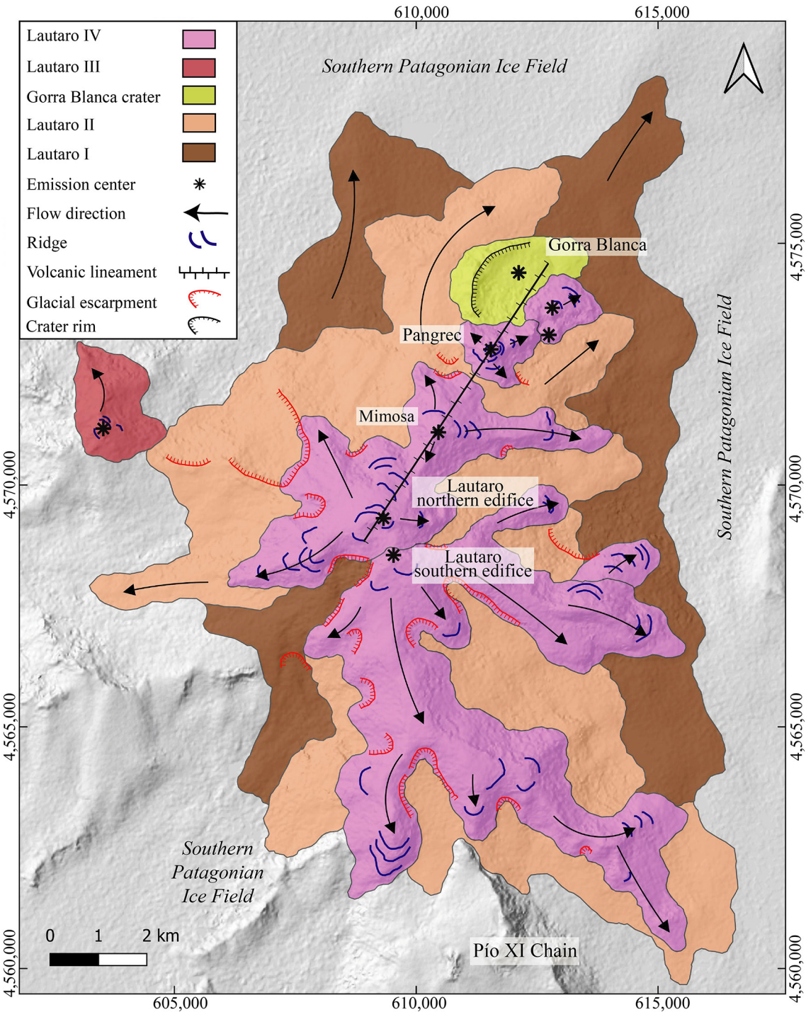
FIG. 6. ALOS PALSAR-derived shaded relief image showing the geomorphological units identified from the RRIM for the Lautaro volcano. See text for explanations.
