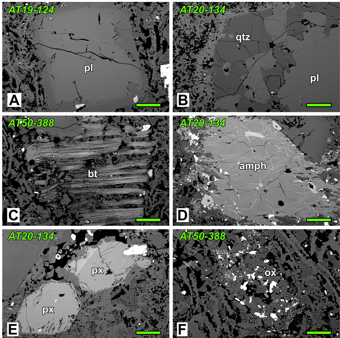
FIG. 4. Backscattered electron images (BSE) of samples from the Patao Ignimbrite. A. Euhedral plagioclase phenocryst developing concentric normal zoning. B. Crystal clotted with anhedronal quartz and subhedral plagioclase. C. Subhedral biotite phenocryst. D. Subhedral amphibole crystal with dehydration rim. E. Pair of euhedral pyroxene phenocrysts. F. Oxide-rich lithic clast. The green line is 100 \mu\text{m} long. The matrix in all the images is composed of microphenocrysts of quartz, plagioclase and glass shards.
