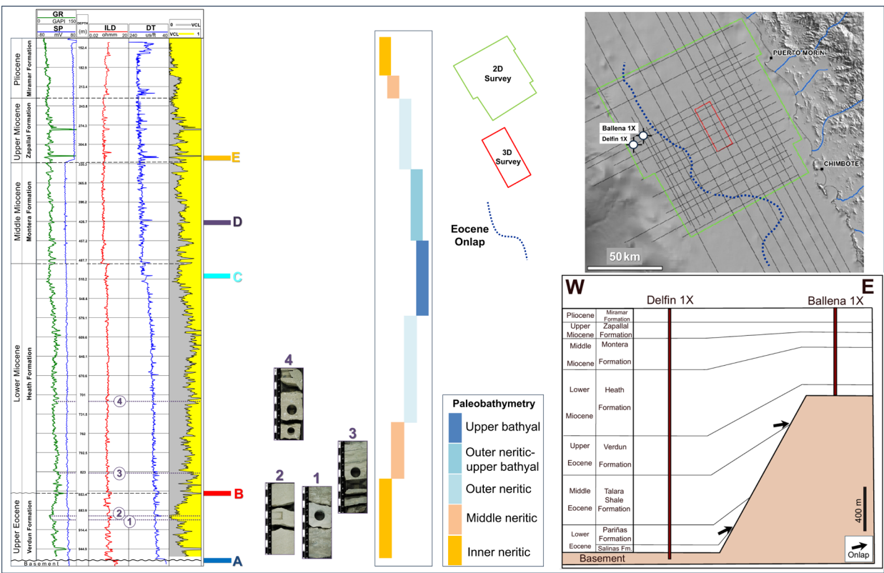
FIG. 3. Trujillo Basin. Ballena 1X well data, adapted from Timoteo (2015) and Timoteo et al. (2018). Well log measurement abbreviations: GR : Gamma Ray (GAPI, Gamma American Petroleum Institute), SP : Spontaneous Potential, ILD : Induction Deep Resistivity, DT : Sonic Transit Time. Color-coded horizontal bars indicate the lower boundary for each depositional sequence (A through E) defined in this study. Note the deepening trend, evidenced by increasing GR, decreasing volume of clay (VCL), and inferred paleobathymetry based on foraminifera (Okada, 1990) and core data analysis. This trend extends from the upper Eocene Verdun Formation through the lower two-thirds of the Lower Miocene Heath Formation. A reversal to a coarsening- and cleaning-upward GR trend (with accompanying decrease in VCL) is observed in the upper third of the Heath Formation and continues through the remainder of the column. The deepening trend reflects a prolonged underfilled stage in the forearc during the Middle and Late Miocene. Eocene onlap mapped on seismic and by well correlation indicates absence of Eocene sediments in the Salaverry Basin. Cores from the Verdun Formation (1, 2) and from the lower half of the Heath Formation (3, 4). 1 : Inner shelf-prodelta fine- to medium-grained sandstone; intensely bioturbated mottled interval; original lamination pervasively disturbed. 2 : Delta front-mouth; planar cross-bedded sandstone and plant debris. 3 : Graded turbidite sandstone beds containing abundant mudclasts at their bases; tops capped by dark, organic-rich claystone. 4 : Graded/stratified, locally diffusely cross-bedded pebbly turbidite sandstone. Inset map shows well locations, the 2D lines (gray network), the extent of the 2D grid incorporated in the evaluation (green contour), the extent of the 3D survey (red rectangle), and the inferred position of the Eocene onlap (blue dotted line). Bottom right: E-W schematic profile obtained after integrating data from the Ballena 1X and Delfin 1X wells. Core description and interpretation after CoreLab (2012) 13 .
