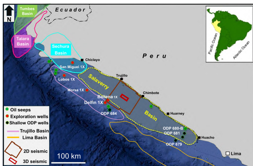
FIG. 1. Map of the forearc basins of northern and central Peru. The oil-producing basins, Talara and Sechura, are located in northernmost Peru and extend both offshore and onshore (Hay-Roe and Miller, 1992; Zuñiga-Rivero et al. , 1998; Higley, 2004; Martínez et al. , 2005 1 ; Fildani et al. , 2005; PeruPetro, 2005 2 ; Daudt and Scherer, 2006; Meza et al. , 2010; Rossello et al. , 2022). The Trujillo, Salaverry, and Lima basins lie entirely offshore. This study focuses on the analysis of 2D seismic data (outlined in brown) and the Chan Chan 3D survey (outlined in red) within the central part of the Salaverry Basin (yellow dashed line). Oil seeps and shallow ODP wells are shown as green and black circles, respectively. Modified from Timoteo et al. (2018).
