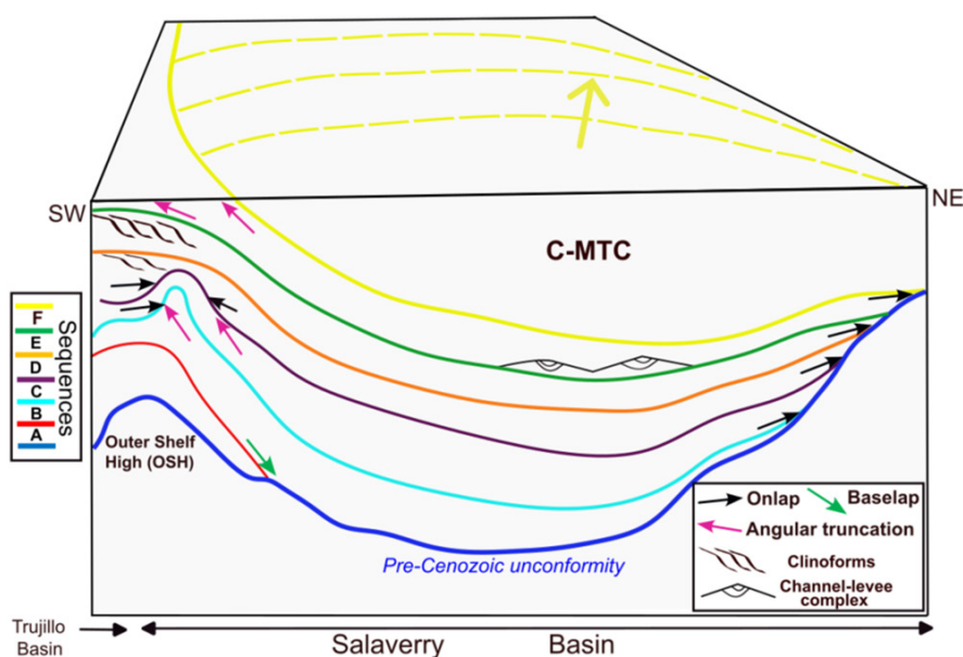
FIG. 18. Summary of key stratal terminations and sequence stratigraphy in the central Salaverry Basin, highlighting two major uplifts affecting its western (seaward) margin: the OSH. The initial phase resulted in the erosion of sequences A and B. Sequence C typically exhibits angular truncation, while sequence D thins and drapes over the OSH, with eastward (basinward) clinoform progradation in its upper section on the eastern OSH flank. Sequence E shows also basinward progradation, as indicated by the presence of clinoforms on the OSH. Sequence F is characterized by substantial thickening over the OSH, with channel levee complexes resting on its lower boundary and entering the basin from the southeast. A subsequent late uplift phase caused tilting and erosion. Northerly clinoform progradation in megasequence C-MTC indicates axial sediment flow in a confined basin. The stratal terminations of sequences B through F along the eastward (landward) basin margin are characterized by progressive onlaps. Sketch interpreted from figure 4. See text for discussion.
