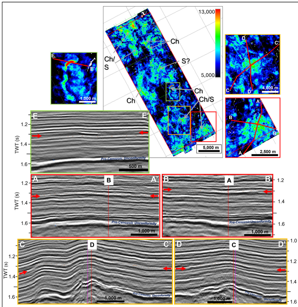
FIG. 13. Root-mean-square (RMS) amplitude map of the depositional elements in sequence C, including splay-like features (S) and channel-like, shoestring forms (Ch). High RMS values are shown in warm colors, while low values appear in cool colors. The 3D survey outline is shown in red, matching the main map. 2D seismic grid shown as gray lines. Inner grid of the 3D and part of the 2D lines used for amplitude map generation shown as thin, faint lines. CHAN denotes the proposed location of a vertical exploration well targeting the Chan Chan trap. Squares in the lower half of the map refer to individual panels A-A', B-B', C-C', and D-D', which represent seismic sections of splay-like elements, and panel E-E', which shows a cross-section of channel-like forms (zoomed-in excerpts showing section locations provided next to the main map). The red vertical lines in some profiles indicate the position of the intersecting profiles. Red arrows indicate horizons for gated (0, -40ms) amplitude extraction. The apex of the Chan Chan trap is displayed on seismic lines C-C' and D-D' by a magenta vertical line. Scale bar as in figure 12B. TWT: two-way travel time.
