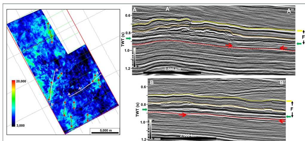
FIG. 14. Root-mean-square (RMS) amplitude map of the uppermost section of sequence E. High RMS values are displayed in warm colors, while low values appear in cool colors. The outline of the 3D survey is shown in red. 2D seismic network shown as gray lines. Inner grid of the 3D and part of the 2D lines used for amplitude map generation shown as thin, faint lines. Purple dot denotes the proposed location of a vertical exploration well targeting the Chan Chan trap. The dashed red lines represent the horizons used to generate the gated (-30ms, +10ms) amplitude map. Green arrows on the seismic cross sections mark the lower boundary of sequence F; the yellow continuous line indicates its upper boundary. Intra-sequence horizon (dashed yellow line) demarks top of mounded geometries in the lower part of said sequence. On the A-A' arbitrary line, the red arrows highlight the length of a potential sand ridge located immediately above the dashed red horizon, whereas on the B-B' line, a similar sand ridge locates immediately below this horizon. Scale bar indicates the polarity of seismic data. TWT: two-way travel time.
