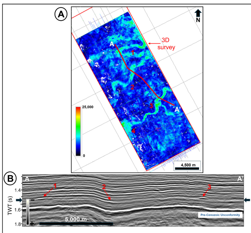
FIG. 11. A. Root-mean-square (RMS) amplitude map of the upper half of sequence B. High RMS values are shown in warm colors, while low values appear in cool colors. The RMS window (-10ms, +30ms) reveals two main channel systems: features 1 and 2, interpreted as segments of a single high-sinuosity system, and feature 3, which appears to terminate in a minor terminal splay or lobe (feature 4 on map). A/B amplitude ratios are relatively low ( \sim 2.3 ) across the channel systems, indicating limited sand development. CHAN denotes the location of a potential vertical exploration well targeting the Chan Chan trap. Outline of the 3D survey in red. 2D seismic network shown as gray lines. The 3D grid and part of the 2D lines used for amplitude map generation shown as thin, faint lines. B. NW-SE oriented A-A' arbitrary line, showing the seismic expression of channels 1-2 and 3. The 1-2 channel system lies just below the reference horizon (black arrows) used in the RMS amplitude map, while channel 3 is slightly above it. Scale bar indicates the polarity of seismic data. TWT: two-way travel time.
