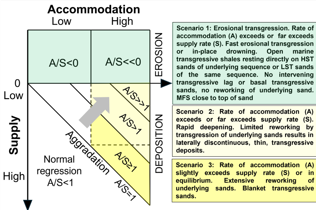
FIG. 10. Depositional models under varying accommodation and sediment supply conditions, after Curray (1964) and Cattaneo and Steel (2003). Transgressive deposits and the preservation of transgressive sands are shown as a function of accommodation rate (A) and sediment supply rate (S). The gray arrow indicates the trend of decreasing sediment supply and increasing accommodation. The Basal Sand Complex is interpreted to have formed during a transitional stage between scenarios 2 and 3. Scenario 3 (blanket transgressive sands) and Scenario 2 (discontinuous transgressive sands) are suggested to prevail south of and on the Chan Chan High. In contrast, Scenario 1, where accommodation rate greatly exceeds supply rate, dominates north of this high, resulting in the absence of transgressive sands and the deposition of fine-grained sediments through suspension settling. HST : highstand systems tract. LST : lowstand systems tract. MFS : maximum flooding surface. See text for details.
