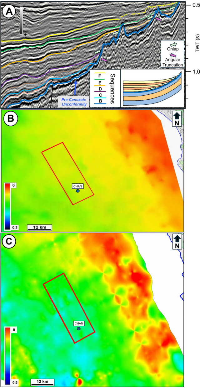
FIG. 8. Stratigraphic terminations along the eastern basin margin. Scale bar indicates the polarity of seismic data. A. Coastal onlap of sequences B-F highlights progressive eastward basin expansion (see scheme). Thinning towards the east, especially for sequences B and E, indicates periods of maximum subsidence. Orange thin lines represent intra-sequence horizons, which also show progressive onlap. B. Isochore map (in seconds) of sequence B. The landward extent of the isochore is extrapolated beyond the limits of the 2D seismic lines. C. Isochore map (in seconds) of sequence D. The coastal onlap of this sequence extends farther landward when compared to the onlap of sequence C (see figure 7); however, due to poor seismic quality, this onlap is not fully captured in the isochore map. Note the smooth eastward thinning of sequence B and the uneven thinning of sequence D due to basement highs. Outline of 3D survey in red. TWT: two-way travel time. CHAN denotes the location of a potential vertical exploration well targeting the Chan Chan trap. See text for details.
