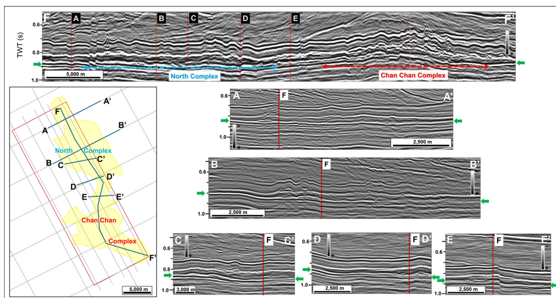
FIG. 15. Channel-levee-fan complexes at the base of sequence F. The outline of the 3D survey is shown in red. 2D seismic grid shown as gray lines. Yellow area on map shows the extent of both channel-levee-fan complexes. Green arrows on the seismic cross sections indicate the basal boundary of sequence F, on which both the North and Chan Chan complexes are developed. The A-A' to D-D' lines show the development and internal architecture of the North Complex. The E-E' line illustrates inter-complex facies toward the SSE where the Chan Chan Complex is located. The F-F' arbitrary 3D line along depositional strike depicts the lateral relationship of both complexes. Inferred paleoflow direction is from SE to NW. The red vertical lines in the profiles indicate the position of the intersecting profiles. The apex of the Chan Chan trap is displayed on F-F' by a magenta vertical line. Scale bars indicate the polarity of seismic data. TWT: two-way travel time.
