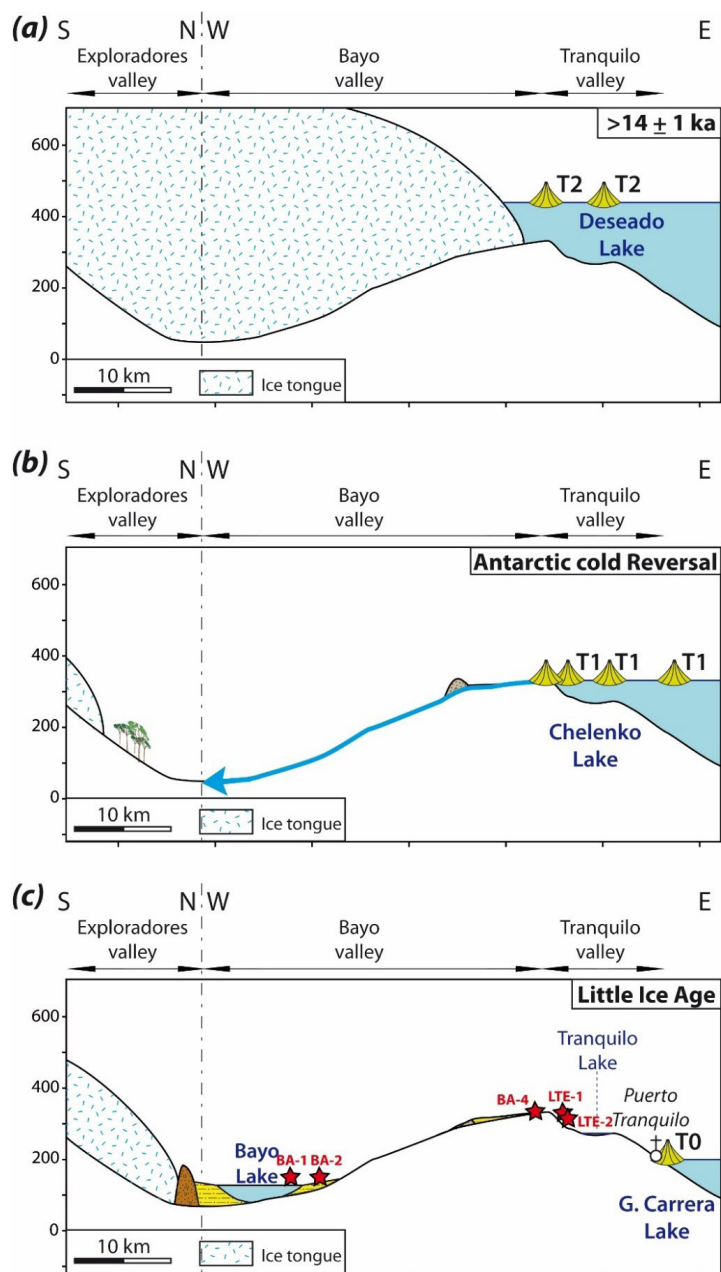
FIG. 8. Conceptual model of the evolution of the BRV in relation to the ice and lake extends. T0 : Recent lake-terraces (210 m a.s.l.). T1 : Chelenko lake-terraces (~350 m a.s.l.). T2 : Deseado lake-terraces (~460 m a.s.l.). Red stars show sites of ^{10}\text{Be} cosmogenic exposure ages.
