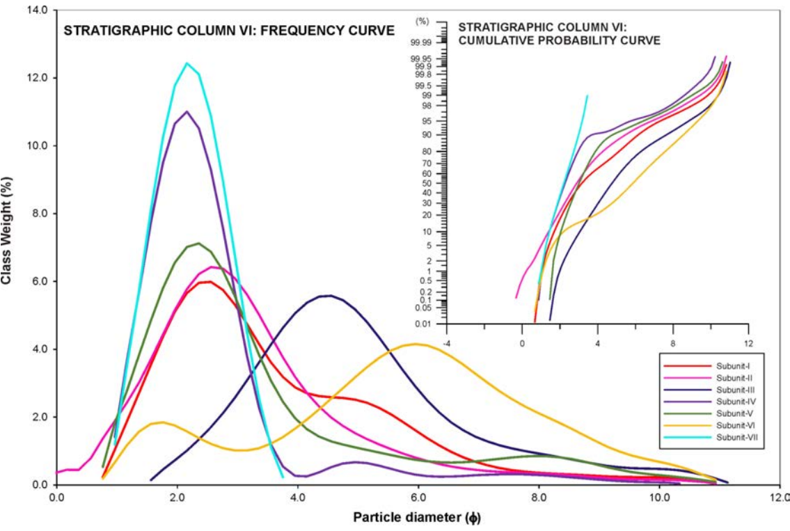
FIG. 2. Frequency and cumulative probability curves of each subunit identified in the stratigraphic column VI. The cumulative probability curves according to (Mycielska-Dowgiało and Ludwikowska-Kędzia, 2011) are first group for all the subunit except for the subunits IV, which indicate an eolian and fluvial-eolian origin respectively. The frequency curves show a unimodal distribution for all subunits except for the subunit IV.
