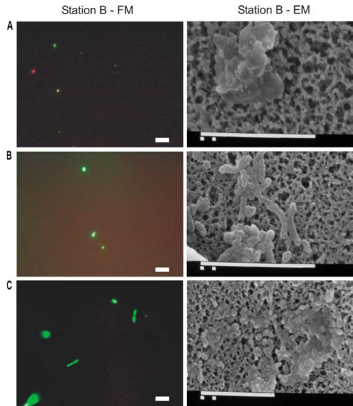
FIG. 5. Fluorescent (left side) and electronic microscopy (right side) of thermophilic and hyperthermophilic microorganisms for bottle samples of Station B. Scale bars indicate 10 μm. A. nk 3: at 1,036 m depth; B. nk 2: at 1,186 m depth; C. nk 1: at 1,036 m depth.
