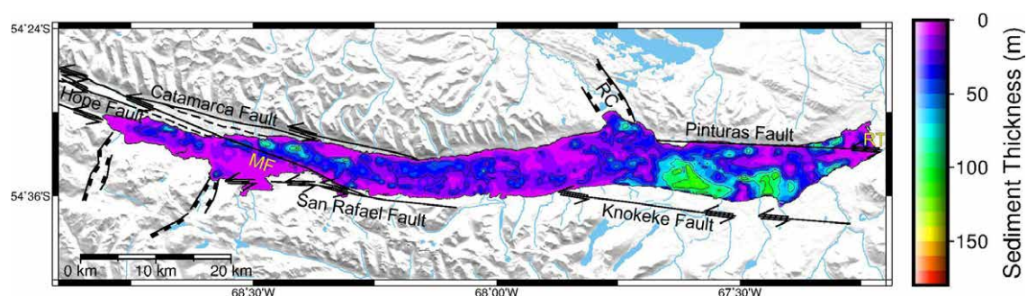
FIG. 9. Glacial isopach map. The sediment thickness was calculated assuming sediment velocity of 1500 m/s. Contour lines (in black) are every 50 meters. MF : Martínez fault; RT : Río Turbio fault; RC : Río Claro fault.
