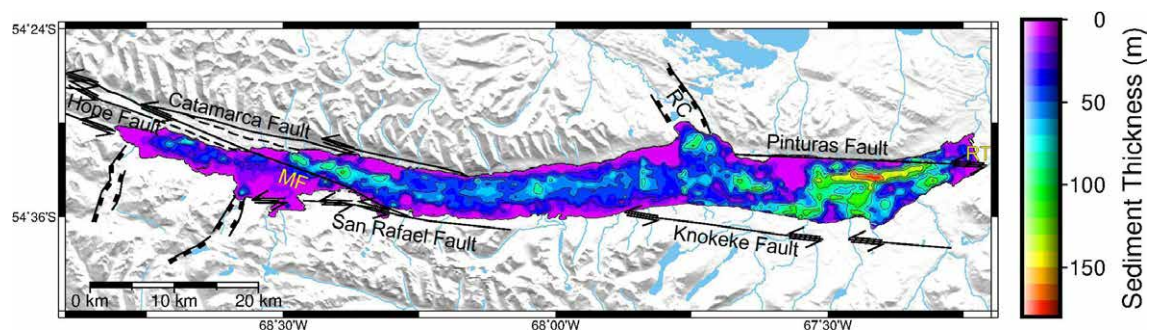
FIG. 8. Total sediment thickness map. The sediment thickness was calculated assuming a sediment sound velocity of 1500 m/s. Contour lines (in black) are every 50 m. MF : Martínez fault; RT : Río Turbio fault; RC : Río Claro fault.
