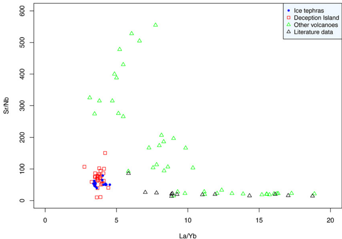
FIG. 24. La/Yb versus Sr/Nb demonstrating that the Livingston Island ice tephrae plot entirely within the field occupied by samples from Deception Island, not overlapping with other volcanic centers. Seal Nunataks literature data taken from Hole (1990) and Hole et al. (1993); Sail Rock literature data from Keller et al. (1992).
