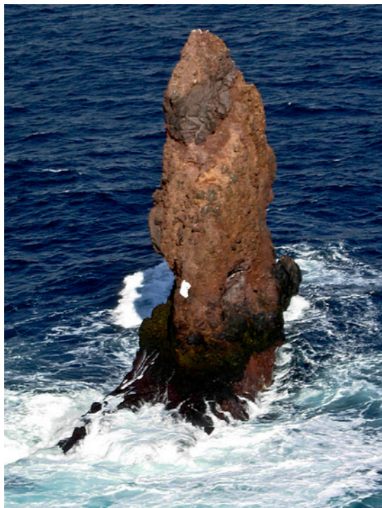
FIG. 2. Sail Rock is the remaining uppermost part of a submerged volcanic edifice, rising ~30 m above sea level. Our sample was taken from a section consisting of interbedded layers of pyroclastic deposits (lighter, reddish parts) and blocks of lava ~1.5 m below the top, underlain by a lava flow (dark brown layer dipping to the left).
