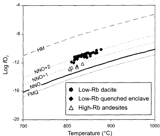
FIG. 13. Temperature versus oxygen fugacity data from magnetite-ilmenite pairs calculated on the basis of the Andersen et al. (1993) algorithm. Oxygen fugacity buffers are FMQ = fayalite-magnetite-quartz; NNO = nickel-nickel oxide; HM = hematite-magnetite.
