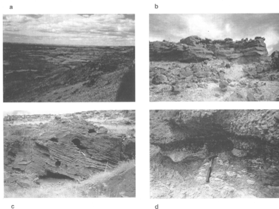
FIG. 4. Las Plumas Member; a - general view of this unit in section A; b - amalgamated coarse sandstones in section A; c - Planar cross-bedded sandstones in section B; d - channels with well-sorted and clast-supported conglomerates in section A.
