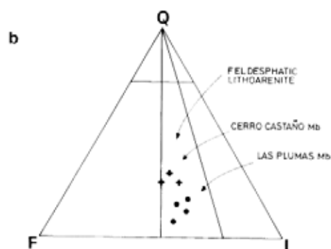
FIG. 6. Triangular diagram for tuffs (Pettijohn et al. , 1987) and QFL diagram for sandstones (Folk et al. , 1970).
