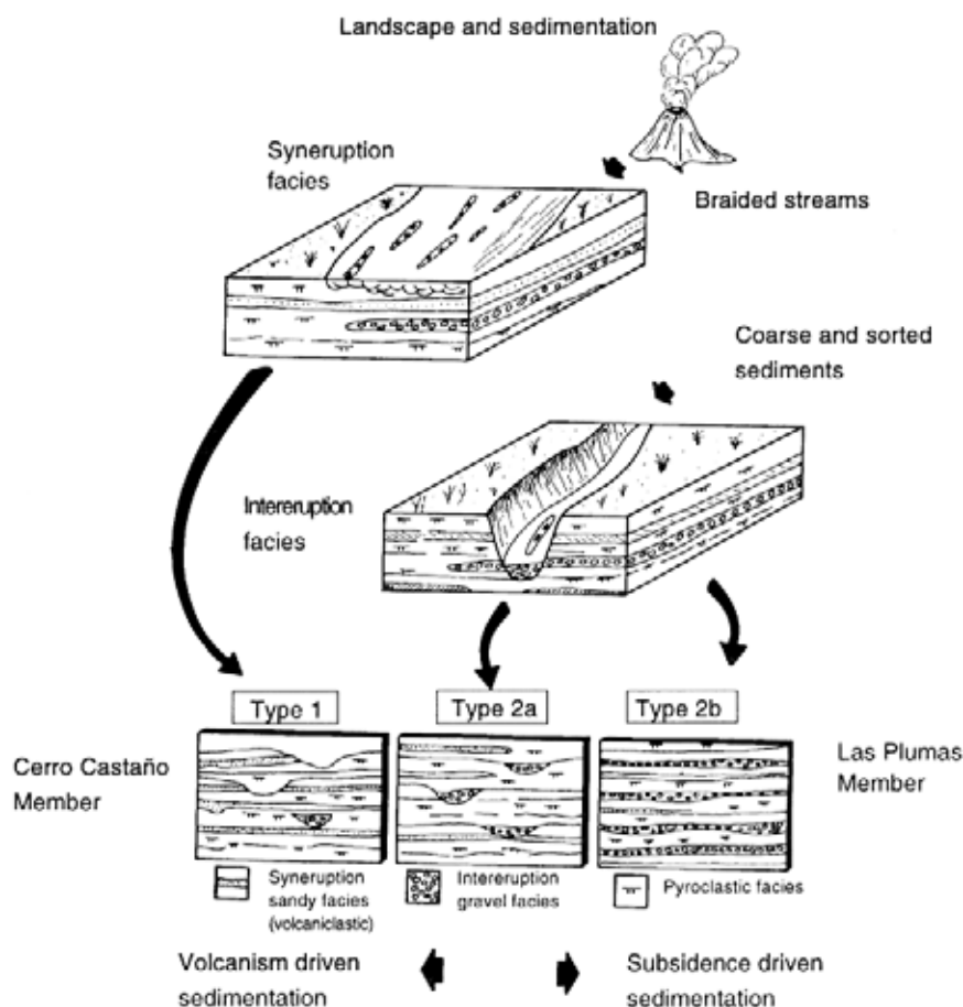
FIG. 10. Block diagrams showing intereruption and syneruption facies within Cerro Castaño and Las Plumas members, adapted from G. Smith (1991).
