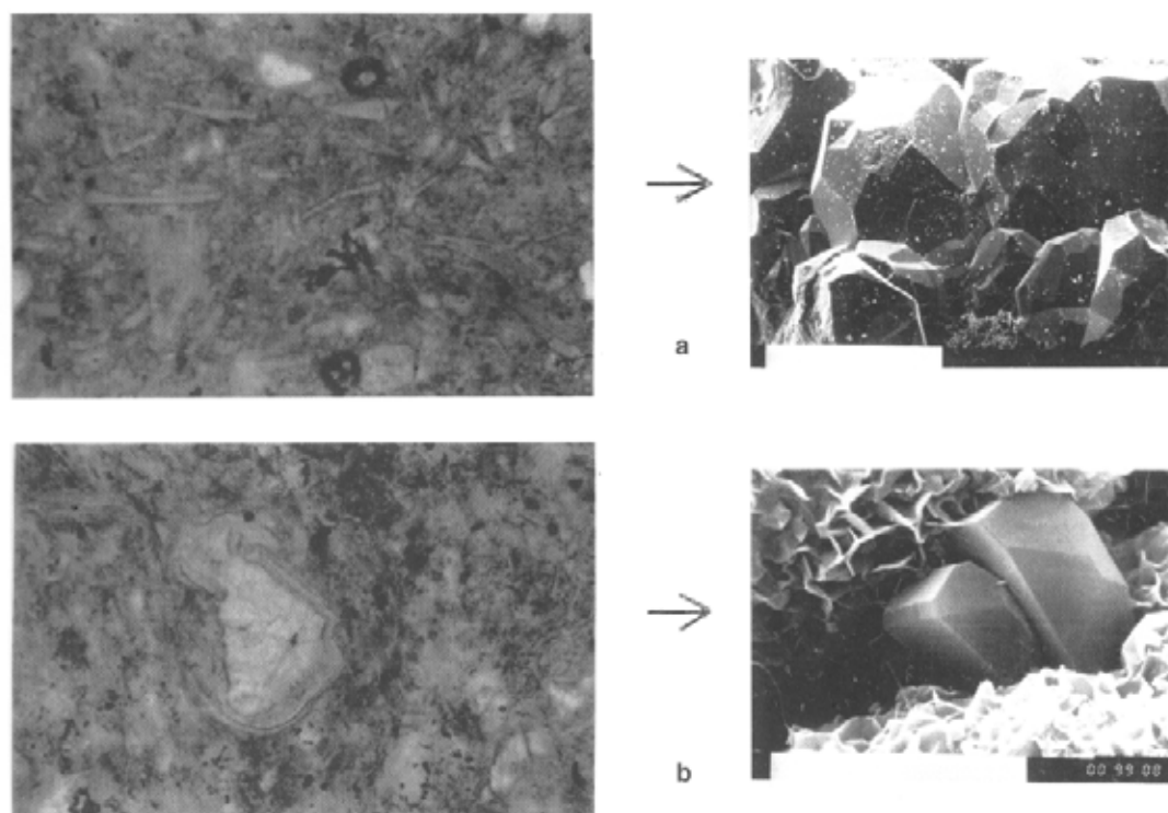
FIG. 7. Optical and SEM pyroclastic petrography; a - vitric-tuff with platy and cusped shards (sample A15) of the Cerro Castaño Member and analcime crystals. b - Vitric-tuff (sample A50) of the Las Plumas Member showing a void successively infilled by smectite-clinoptilolite-mordenite.
