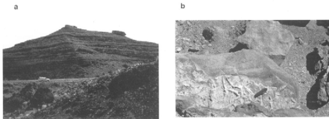
FIG. 3. Cerro Castaño Member; a - general view of the unit in section E; b - trace fossils ( Palaeophycus ) in section B.
