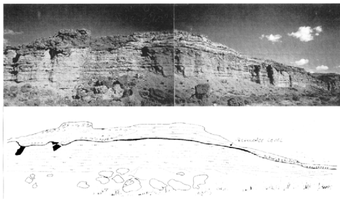
FIG. 5. Erosive surface at the base of the Las Plumas Member. Outcrop view of section B (Fig. 2), amalgamated and tabular conglomerates intercalated with the tuffs.
