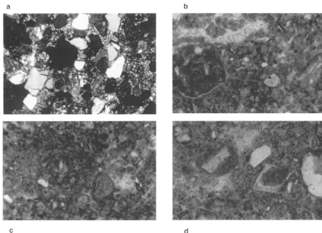
FIG. 8. Las Plumas volcaniclastic lithofacies: a - coarse sandstone with sanidine, quartz and volcanic rock fragments; b - reworked andesitic fragment and veins infilled with zeolite (sample A45*); c - clay rims (cutans) around volcanic rock fragments (sample A 45); d - Diagenetic alteration of detrital plagioclase to clay minerals and lithic fragments (sample A45).
