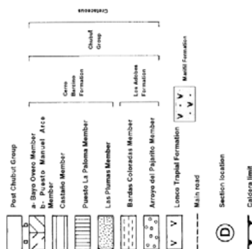
FIG. 1. Geological map with location of studied section and simplified stratigraphic scheme (adapted from Codignotto et al. , 1978).
