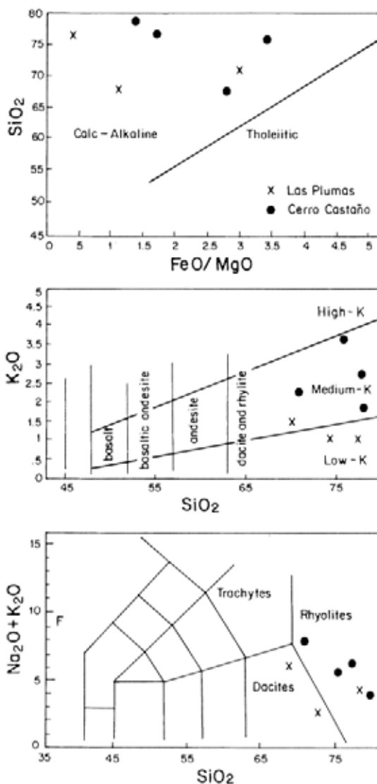
FIG. 9. Discrimination diagrams from Le Maitre et al. (1997). Oxides in weight %. ● = Cerro Castaño Member; x = Las Plumas Member.
